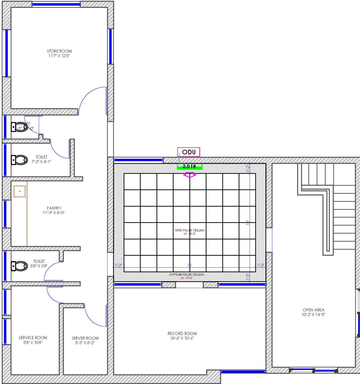
FIRST FLOOR AC LAYOUT
