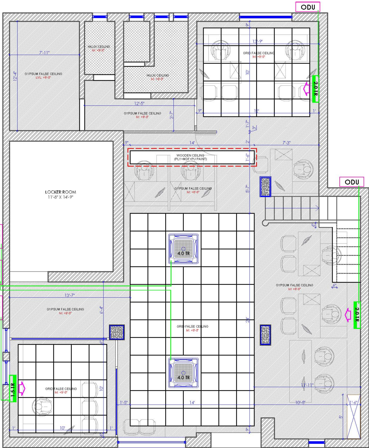
GROUND FLOOR AC LAYOUT
